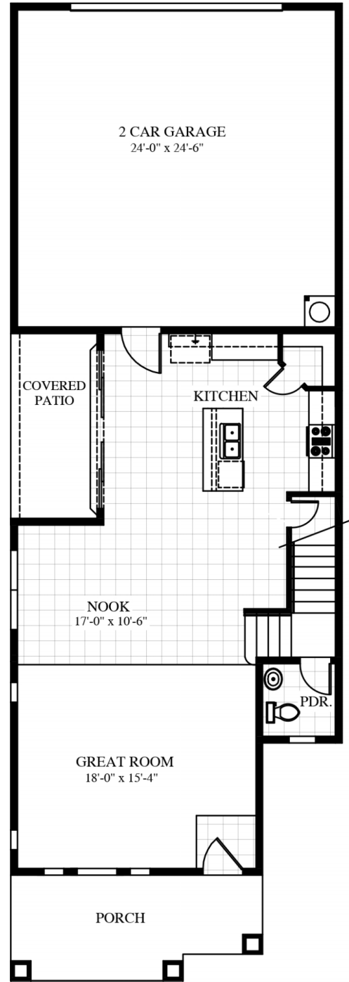
FIRST FLOOR
