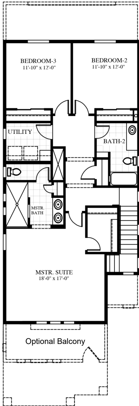
SECOND FLOOR
