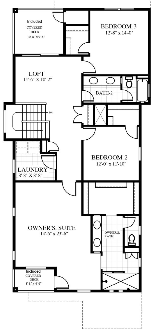
SECOND FLOOR
